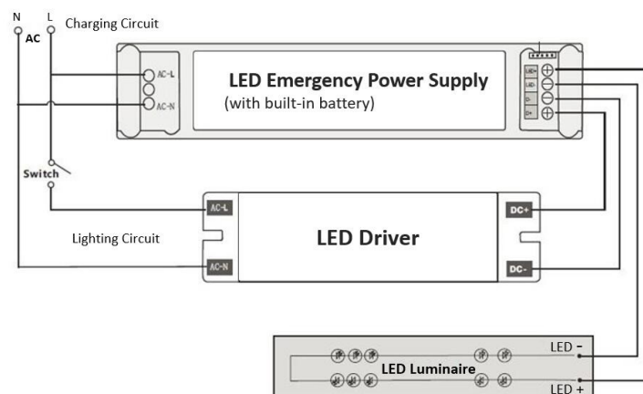
Connection Diagram
